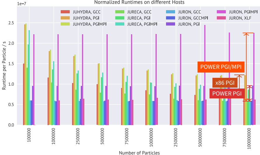
Normalized Runtimes on different Hosts
